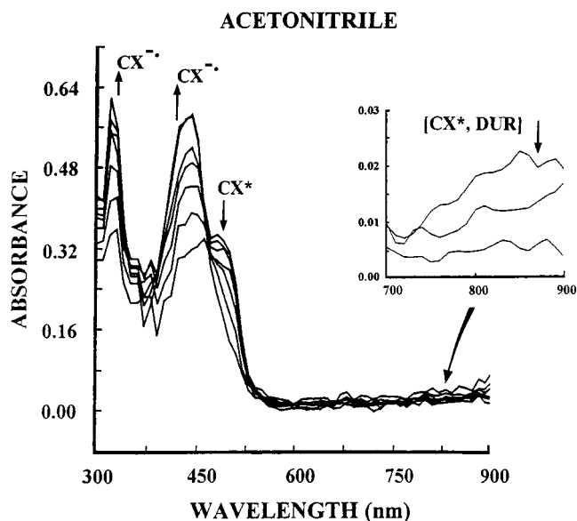
Figure 4. Transient absorption spectra from 0.002 M CX and 0.04 M DUR in acetonitrile following the 10-ns laser excitation at 355 nm. The absorption bands of CX* with \lambda_{\text{max}} = 500 nm and [CX*, DUR] at \lambda > 700 nm (see inset) decayed with the same rate constant ( k = 5.4 \times 10^7 \text{ s}^{-1} ) as the first-order appearance of CX - at \lambda_{\text{max}} = 330 and 430 nm.
