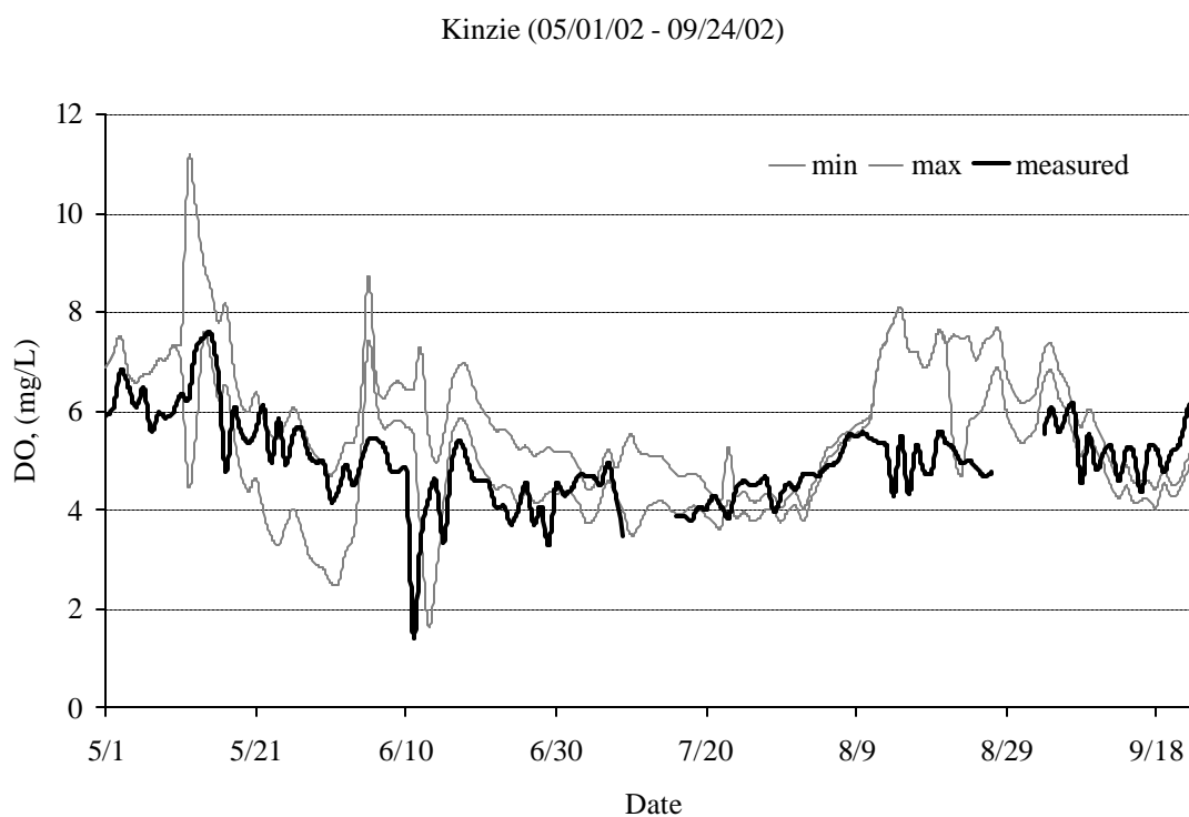
Figure 6.1 Range of simulated dissolved oxygen (DO) concentrations at Kinzie Street on the North Branch Chicago River obtained by Latin Hypercube sampling of storm event mean concentrations compared with the measured DO concentration
