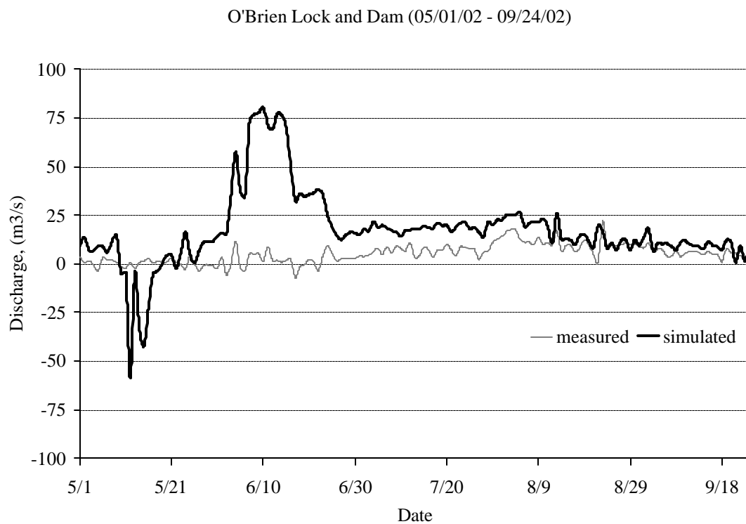
Figure 4.3 (cont.) Comparison of measured and simulated average daily flows at some locations on Chicago Waterway System
