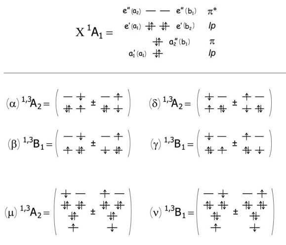
FIG. 2. Leading electronic configurations of the ground (top panel) and the lowest excited states (lower panel). HOMO→LUMO excitations give rise to four singlet and four triplet CSFs labeled \alpha , \beta , \gamma , and \delta . HOMO-2→LUMO excitations yield two additional CSFs of each multiplicity: ( \mu ) and ( \nu ).
