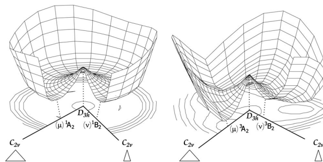
FIG. 5. Adiabatic potential energy surfaces and contour plots of the (\mu)A_2 and (\nu)B_1 singlet (left) and triplet (right) states. Polar radius and angle are hyperspherical coordinates \theta and \phi , which are similar to the bending and asymmetric stretch normal mode, respectively. Stereographic projection is taken with fixed hyperradius (overall molecular size or symmetric stretch) \rho=3.262 corresponding to the cyclic N_3^+ ground state equilibrium geometry. Both surfaces feature conical (\mu)A_2/(\nu)B_1 intersection at D_{3h} . Stationary points on the surfaces are located along two C_{2v} distortions to acute and obtuse isosceles triangles. Energies of the transition state and the conical intersection relative to the minima are E_{TS}=0.05 eV, E_{CI}=0.97 eV and E_{TS}=0.24 eV, E_{CI}=1.03 eV on the singlet and triplet (\mu/\nu) PESs, respectively.
