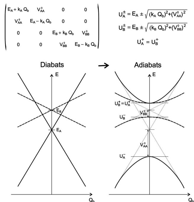
FIG. 8. The Hamiltonian in the diabatic (left) and adiabatic (right) representations along the bending normal mode Q_b . Since the Hamiltonian is block diagonal, the pairs of states of the same symmetry do not interact with each other and form two noncrossing pairs (see text).
