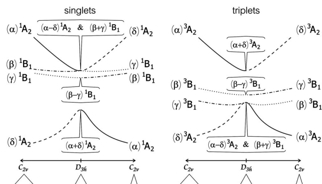
FIG. 3. Changes in the excited states' characters and potential energy surfaces upon distortions from an equilateral ( D_{3h} ) geometry to an obtuse (left) and an acute (right) isosceles C_{2v} triangles.
