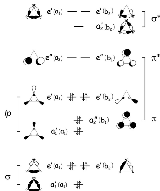
FIG. 1. Molecular orbitals and the ground state electronic configuration of cyclic N_3^+ (equilateral triangle, D_{3h} ). Both HOMO and LUMO are doubly degenerate. C_{2v} labels are given in parentheses.
