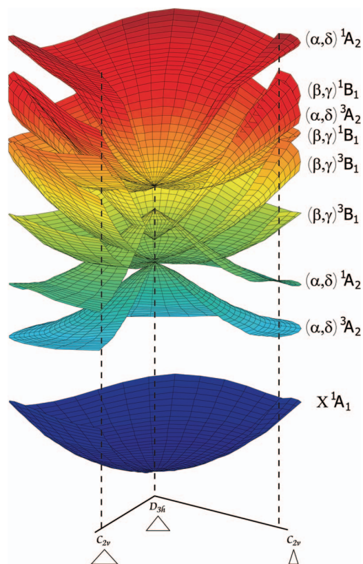
FIG. 6. (Color) PESs of the ground ( X ) and the first eight excited states of cyclic N_3^+ . Coordinates are as in Fig. 5. Three out of four states in each multiplicity are almost degenerate at D_{3h} geometry, two being exactly degenerate.
