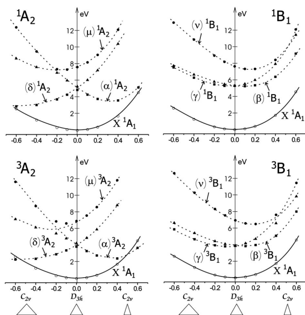
FIG. 4. The EOM-CCSD/6-311G* potential energy surface scans along the bending normal coordinate for the ground ( X {}^1A_1 , shown on each plot) and the excited {}^1A_2 , {}^1B_1 , {}^3A_2 , {}^3B_1 states of cyclic N_3^+ (upper left, upper right, lower left, and lower right, respectively). Data points (squares, triangles, and filled circles) correspond to the calculated adiabatic surfaces; dashed lines represent approximate diabats and connect points with the same leading character of the wave function (see Fig. 2).
